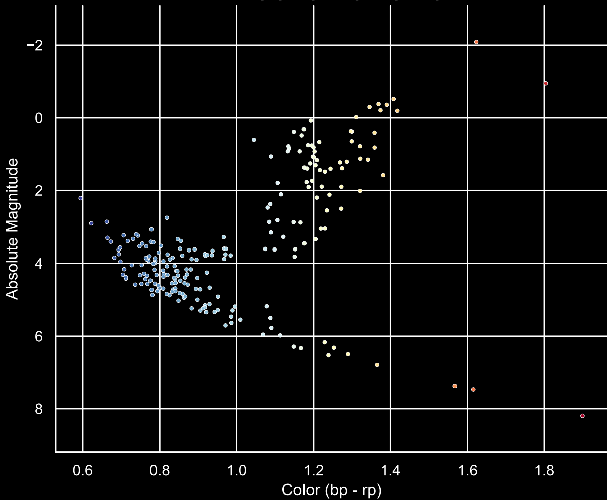
GALAH Hertzsprung-Russell Diagram Field [83] Ra [322.75] Dec [-58.88]
