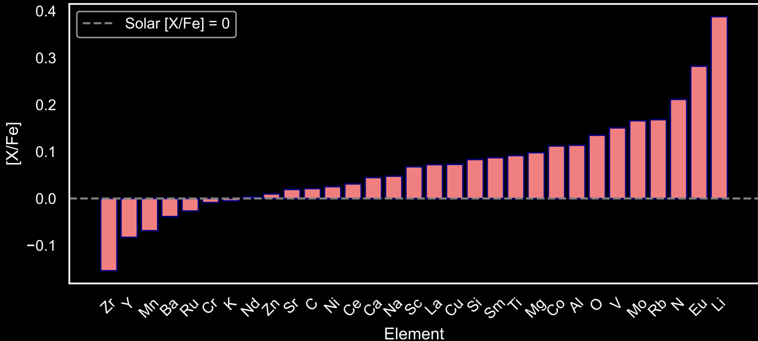
Abundance Pattern for GALAH Star Field [83] (N=223)
