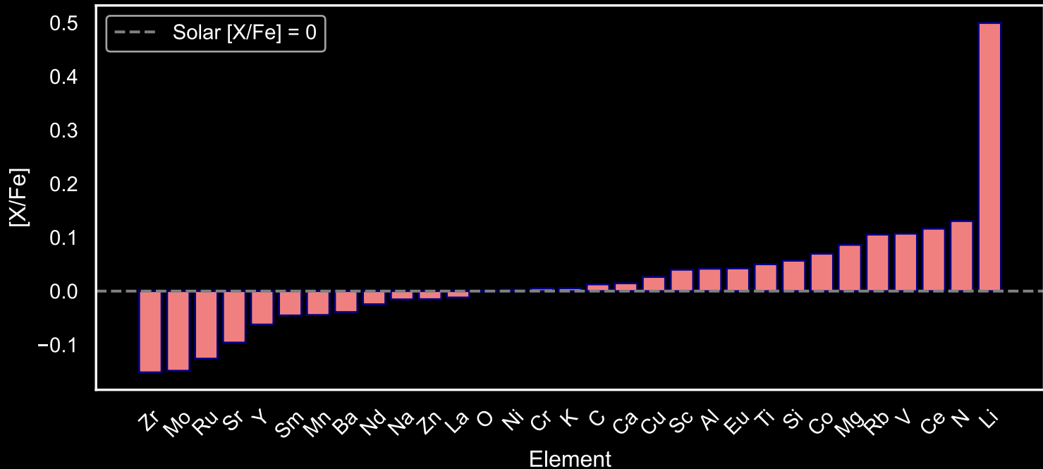
Abundance Pattern for GALAH Main Sequence Stars: Star Field [83] (N=90)
