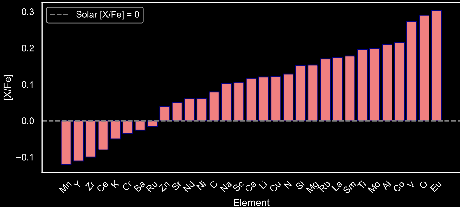
Abundance Pattern for GALAH Red Giants: Star Field [83] (N=69)
