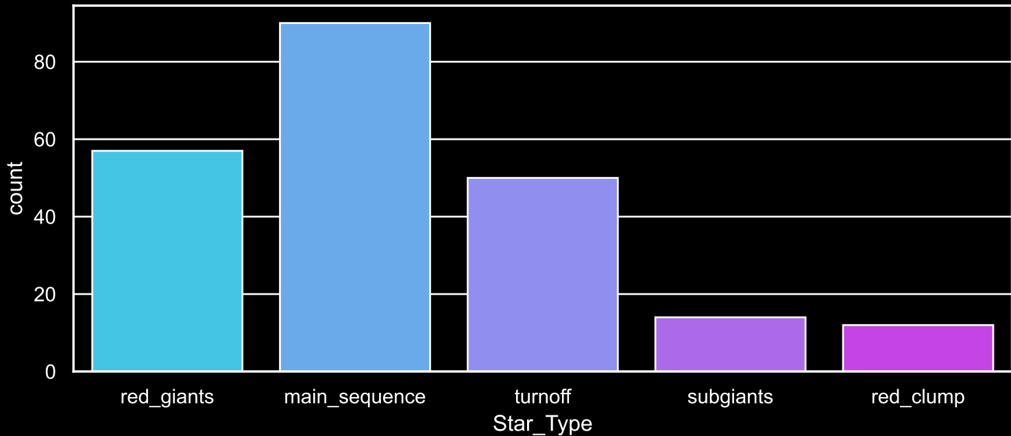
Field [83] Count plot of Star Type
